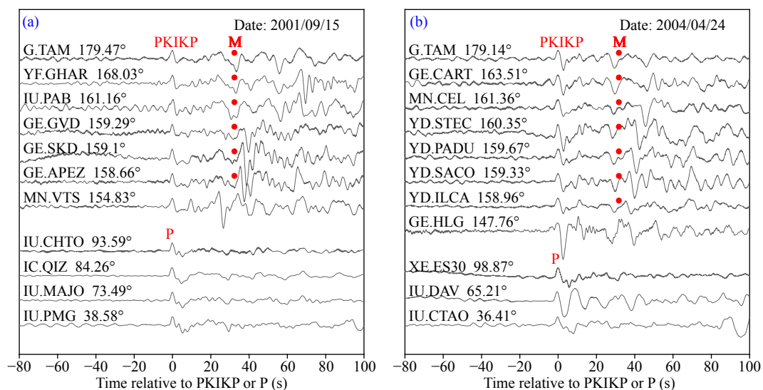
Figure 4. Record sections of two anomalous events, one from Group B (a) and the other from Group A (b). These two events are among the four events in BT10. Seismograms are aligned with PKIKP or P, and high-pass filtered at 100 s to match the previous observations as in BT10. The red dots indicate the M phase. The station name, network code, and epicentral distance are labeled.
