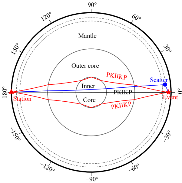
Figure 1. Ray paths of seismic phases passing through inner core, PKIKP (black), PKIIKP (red), and scattered PKIKP (blue) waves.
